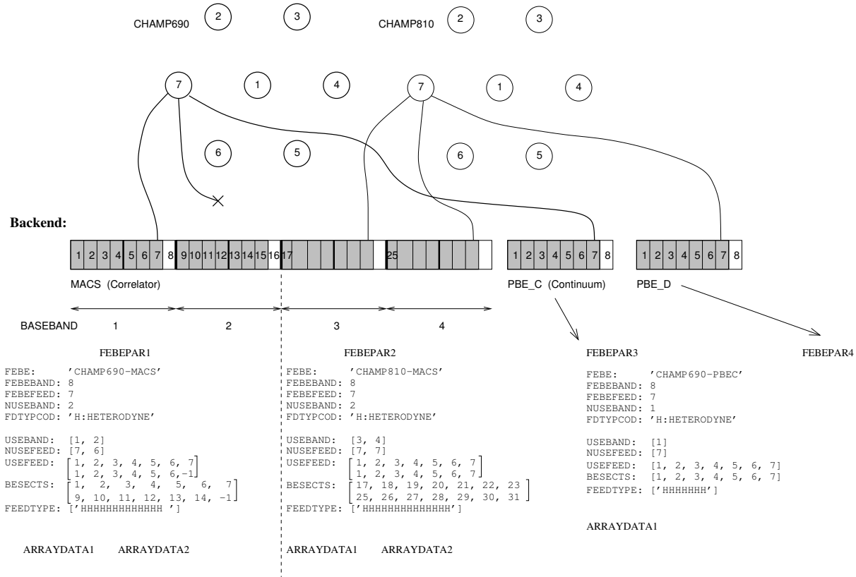
Figure 3: Example FEBE setup showing the values of keywords in the FEBEPAR header and binary table. In this case there are 2 frontends each with 7 physical pixels. Each pixel is connected to 2 correlator bands and a continuum backend (used backend sections shown in grey). This results in 4 different FEBE combinations (therefore 4 FEBEPAR tables). The two correlator FEBEs each have 2 basebands (therefore 2 ARRAYDATA tables). The correlator can only be configured in groups of 4 sections (hence the maximum number of bands is 8). In the case of CHAMP690 , pixel 7 is not connected to the second correlator band. Therefore the corresponding entries in USEFEED and BESECTS are set to -1.
